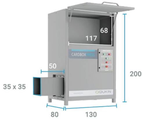
CARDBOXPRESS 200 WITH A LID
