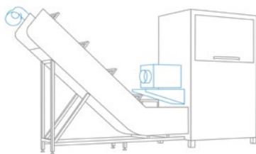
Output transport channel for direct loading into a 1100L container with dust particle filtration system
