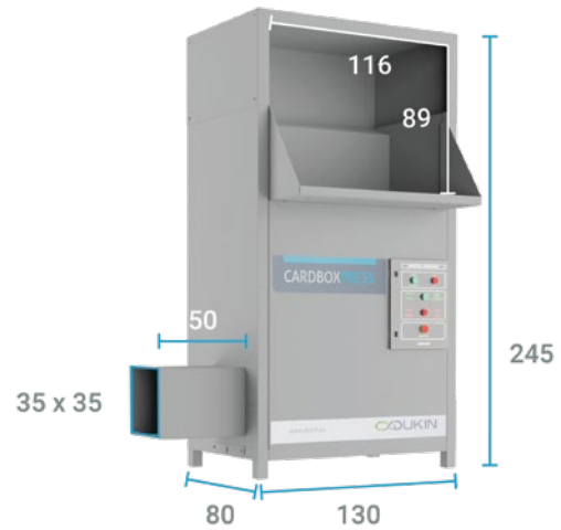
CARDBOXPRESS 200 WITH LOADING OPENING
